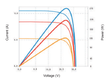
Current-Voltage & Power-Voltage Curve
